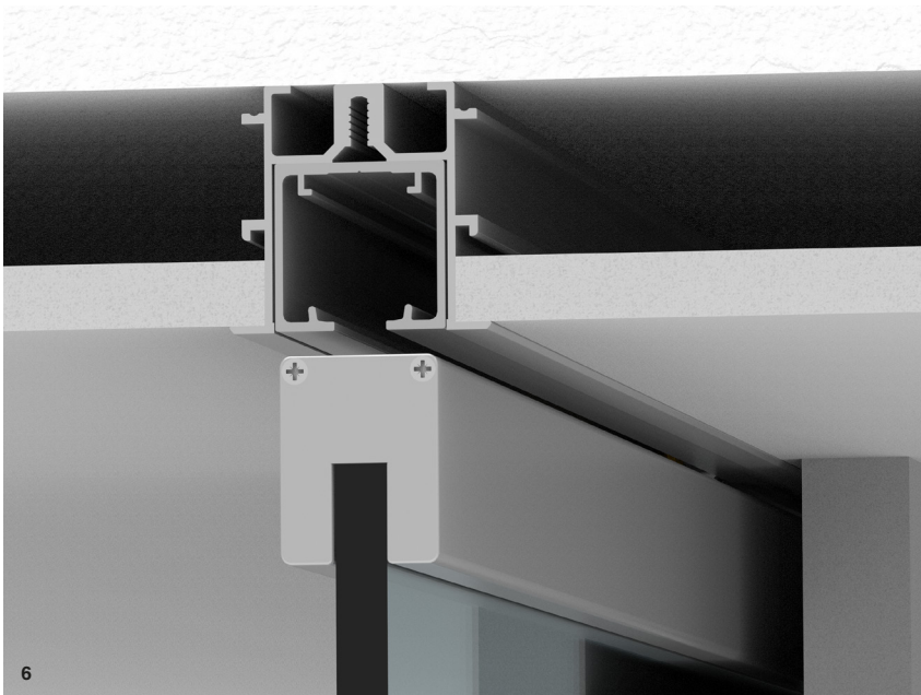
1, 2 y 3 Conjunto perfil Funda FT + Perfil Star, montaje a falso techo I Support FT + Star track set, false ceiling mounting I Ensemble Rail de couverture FT + Star, fixation a faux-plafond. 4, 5 y 6 Conjunto perfil Funda FT + Perfil Star, montaje entre paredes I Support FT + Star track set, mounting between walls I Ensemble Rail de couverture FT + Star, fixation entre les murs.
