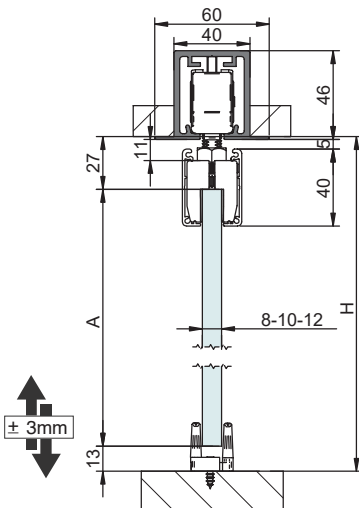
STAR FT XL
