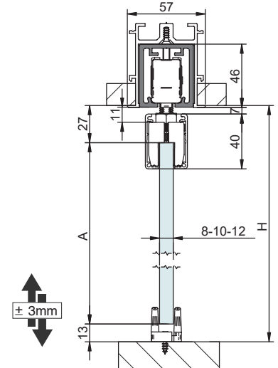
FUNDA FT | SUPPORT FT | COUVERTURE FT XL
