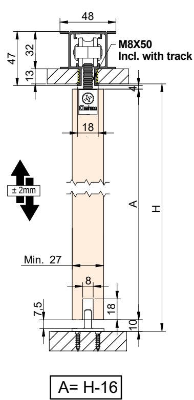
PERFIL STAR FTI FALSO TECHO INVISIBLE Star Track FTI False Ceiling Invisible
