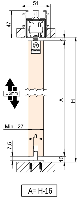
PERFIL FUNDA + STAR FALSO TECHO SUPPORT TRACK + STAR False techo
