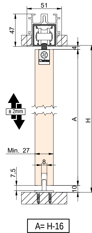
PERFIL FUNDA + STAR FALSO TECHO SUPPORT TRACK + STAR Falso techo
