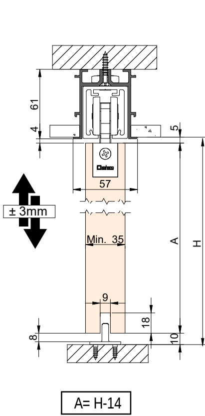
PERFIL FUNDA XL + STAR XL FALSO TECHO SUPPORT TRACK XL + STAR XL False Ceiling
