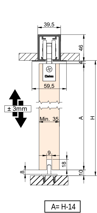
PERFIL STAR FT XL FALSO TECHO /Star Track False Ceiling
