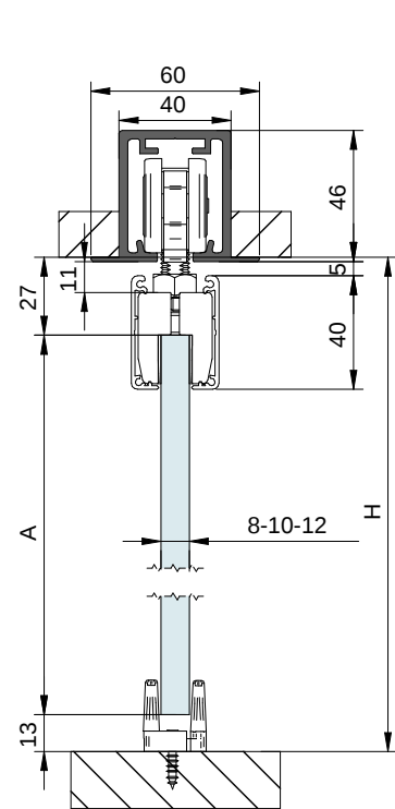
PERFIL STAR a techo STAR Track ceiling mount
