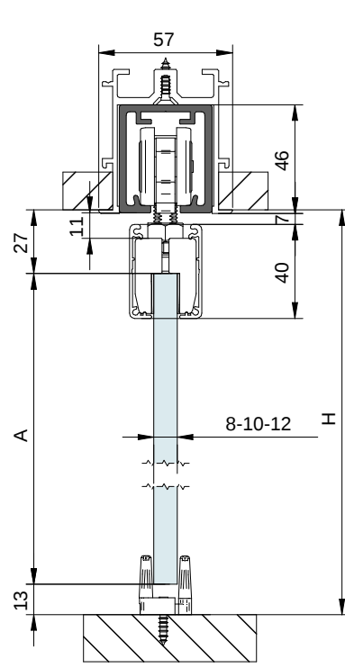
PERFIL STAR FTI FALSO TECHO INVISIBLE Star Track FTI False Ceiling Invisible
